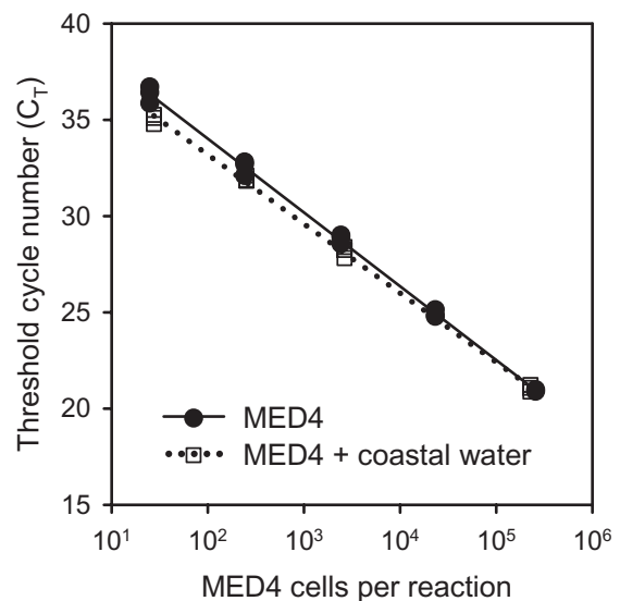
Fig. 3. Comparison of real-time PCR standard curves of MED4 standards (MED4) to MED4 cells spiked into water collected off of the dock at Woods Hole, MA (MED4 + coastal water). Standard curves of triplicate reactions with linear regressions are shown.
