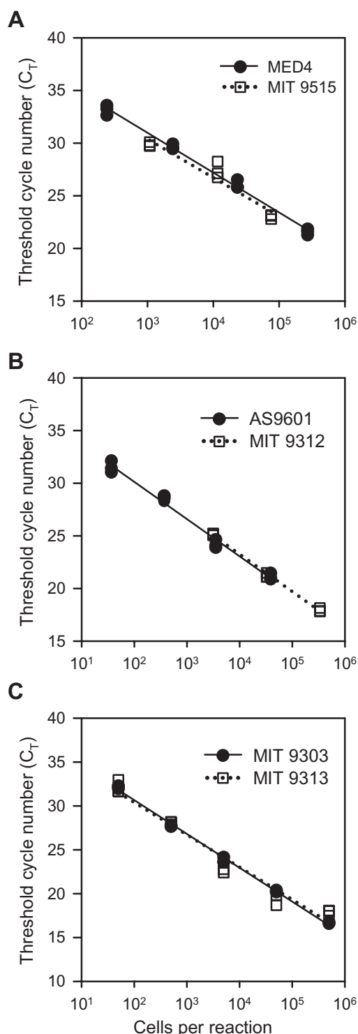
Fig. 1. Threshold cycle number ( C_T ) as a function of amount of template added (cells per reaction) as measured by real-time PCR. The standard curves (cells per reaction versus C_T ) for genomic DNA standards are compared between two strains within an ecotype: (A) strains MED4 and MIT 9515 from ecotype eMED4, (B) strains AS9601 and MIT 9312 from ecotype eMIT9312, (C) strains MIT 9303 and MIT 9313 from ecotype eMIT9313. Points represent triplicate reactions at each concentration tested, and linear regressions of each set of standards are plotted.
