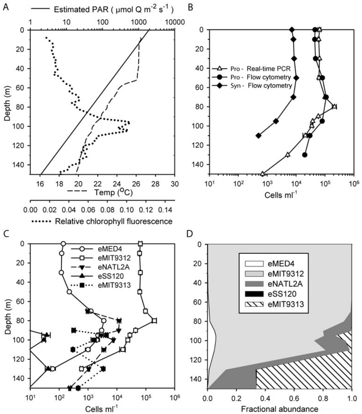
Fig. 5. Depth profiles of hydrographic data and Prochlorococcus abundance from a stratified water column in the Sargasso Sea, September 2001. A. Water column properties.
