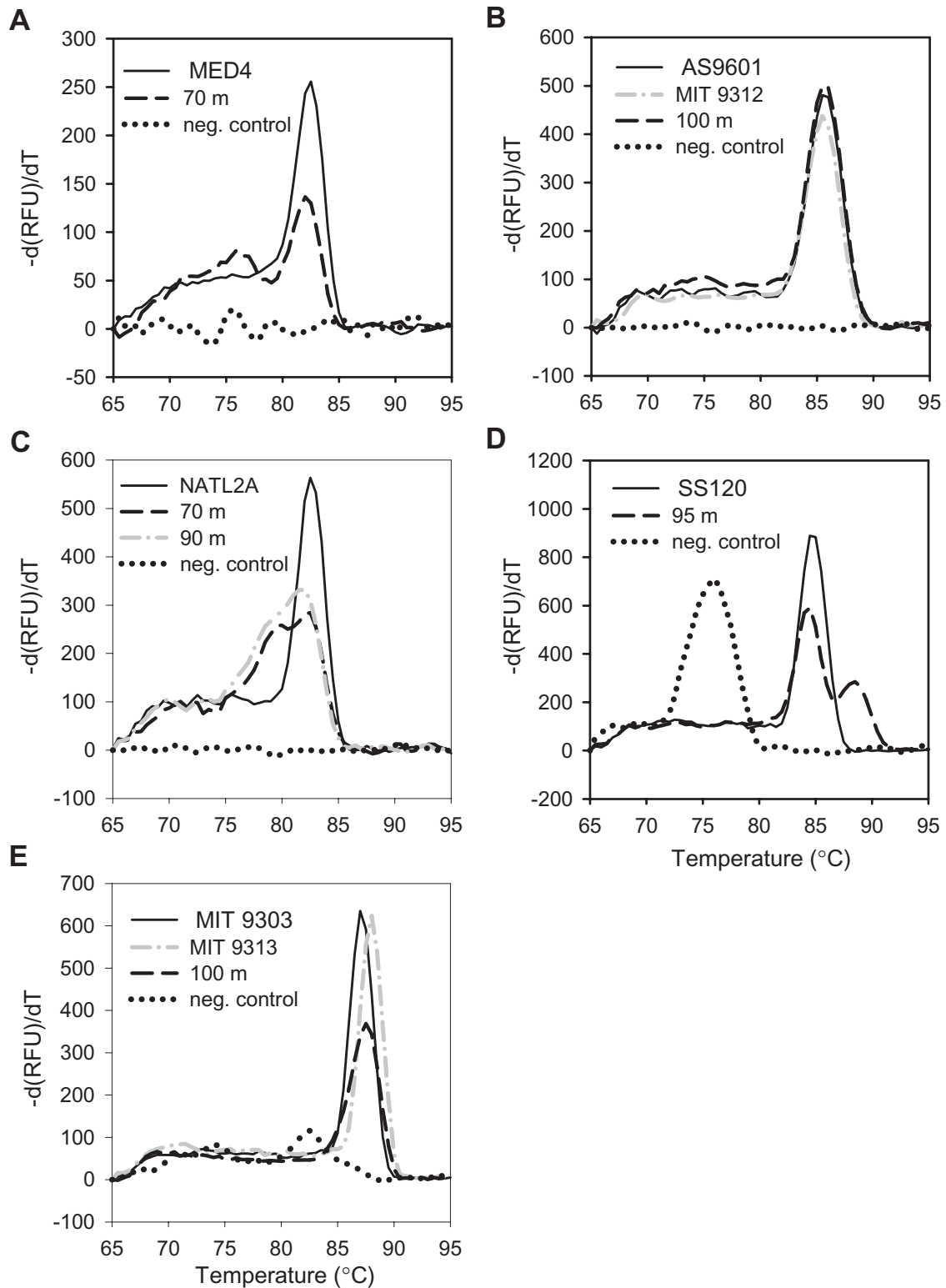
Fig. 4. Representative melting curves of real-time PCR products for standards (solid or dash-dot lines), no-template negative (neg.) controls (dotted lines) and field samples (dashed or dash-dot lines) from the North Atlantic at given depths. The y-axis is the negative of the first derivative of relative fluorescence units (RFU) versus temperature (T). (A) eMED4, (B) eMIT9312, (C) eNATL2A, (D) eSS120, (E) eMIT9313.
